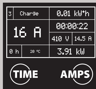
SECTRON AC CHARGER SECTRON BASIC
